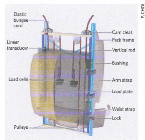
Figure 1 | Suspended-load ergonomic backpack. The pack frame is fixed to the body but the load, mounted on the load plate, is suspended by elastic bungee cord(s) from the frame (shown in light blue and gold). The tension in the elastic cord is set by cam cleats on the top of the frame. When the backpack's locking mechanism is disengaged, the suspended load is free to ride up and down on bushings constrained to vertical rods during walking or running; locking prevents movement and the backpack behaves like a normal rigid backpack. For movies, see supplementary information.
